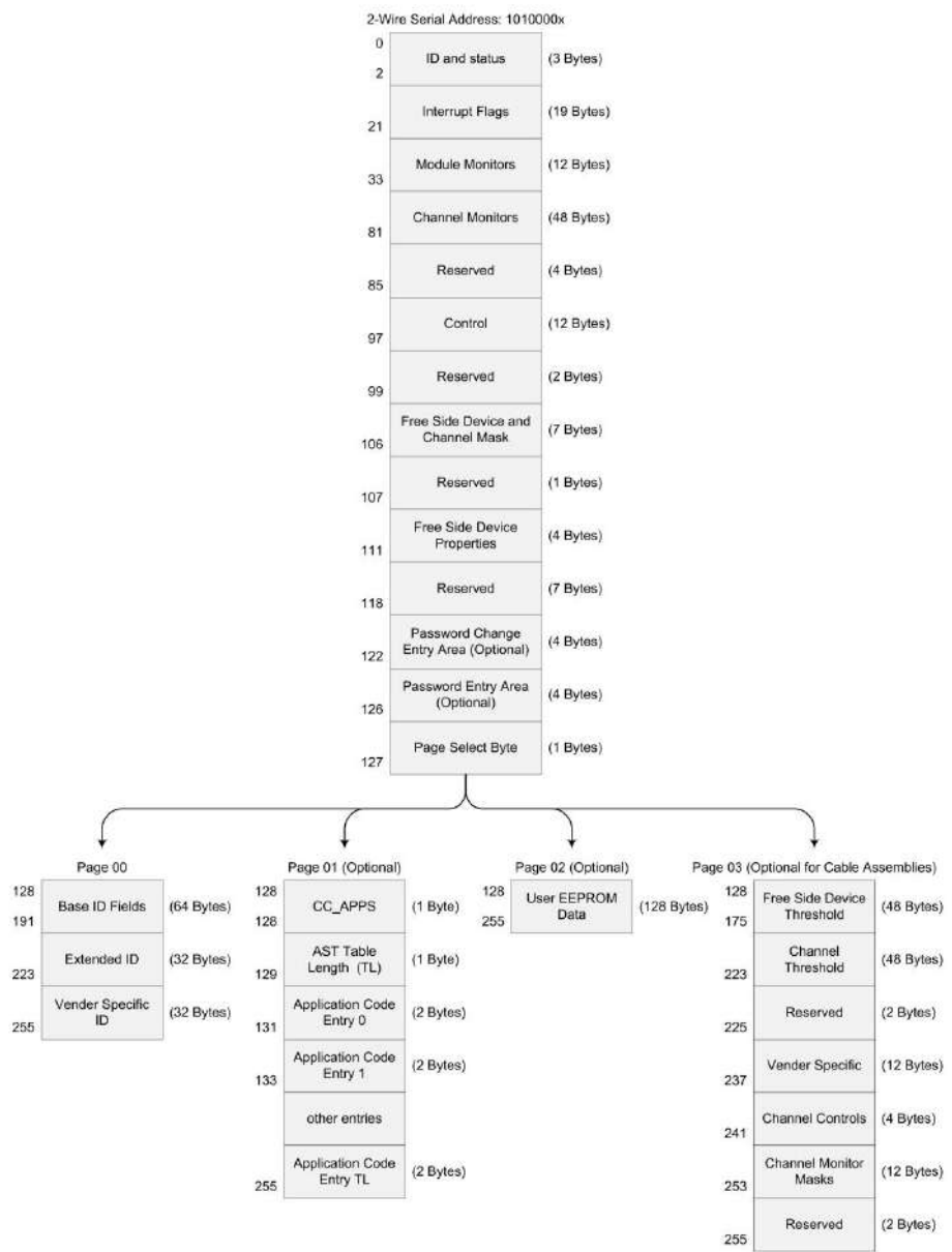
Figure5:Memory map
