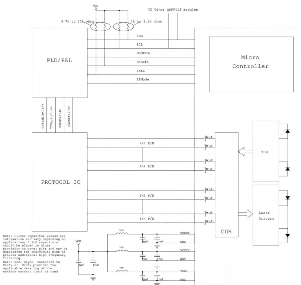
Figure 2: Recommended Interface Circuit
