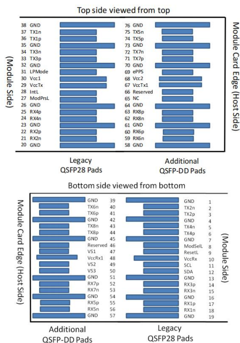
Figure4:Pin view
