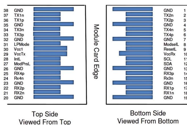
Figure4:Pin view
