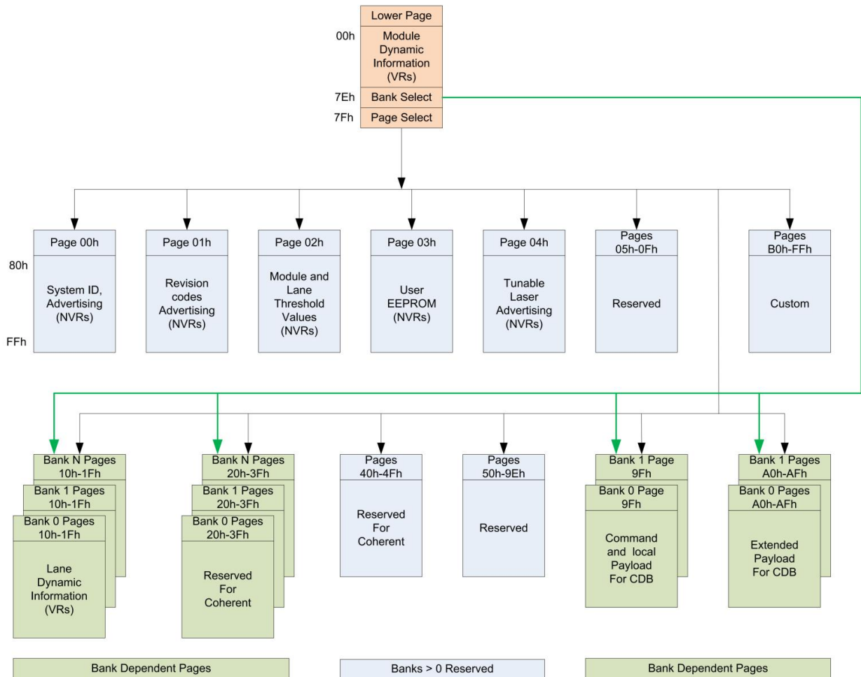
Figure5:Memory map
