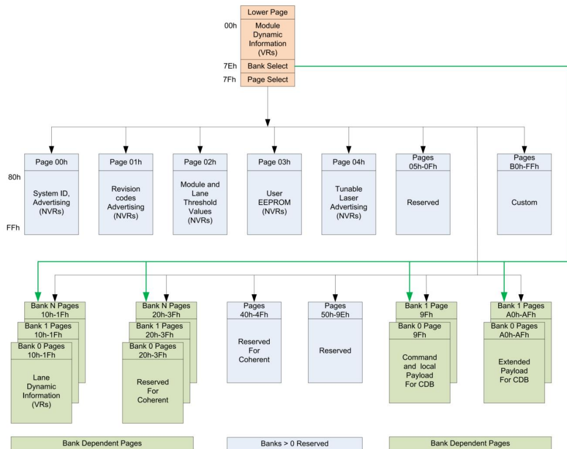
Figure5:Memory map
