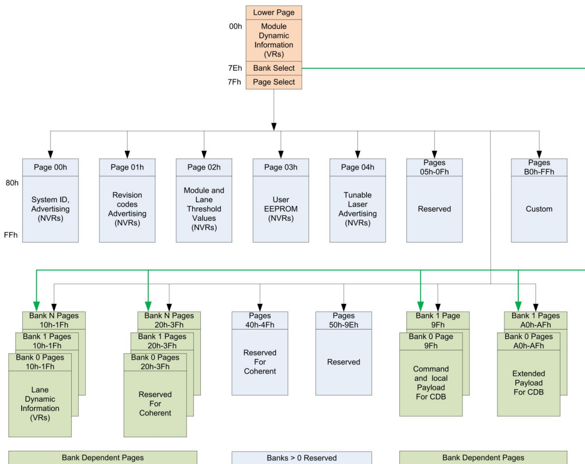
Figure5:Memory map
