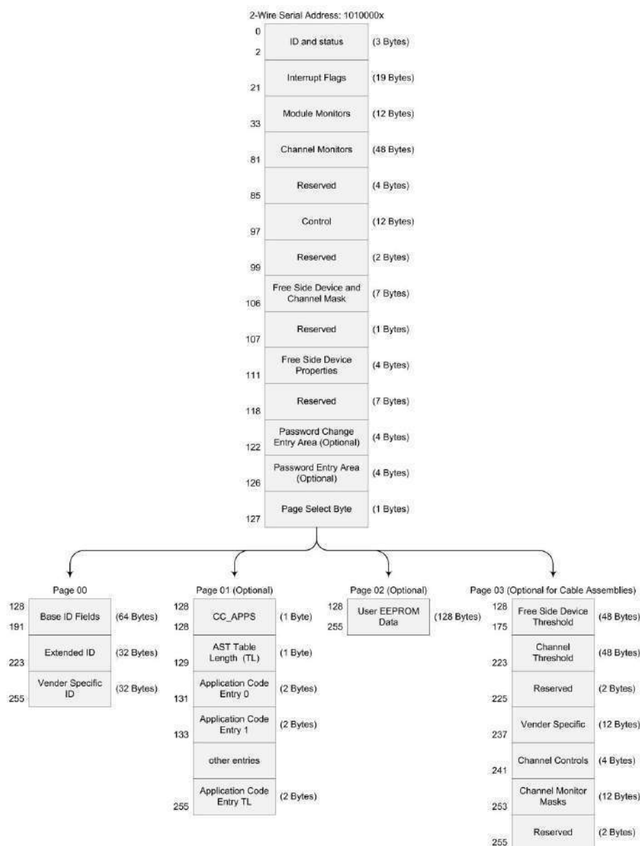
Figure4:Memory map
