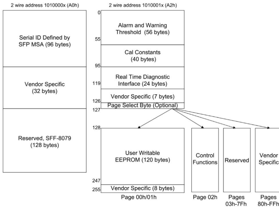
Figure4:Memory map
