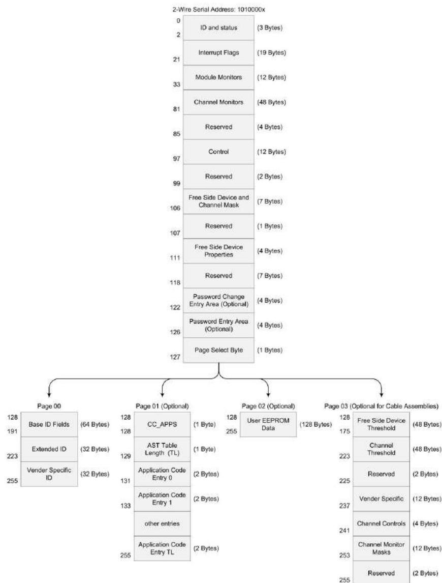
Figure4:Memory map
