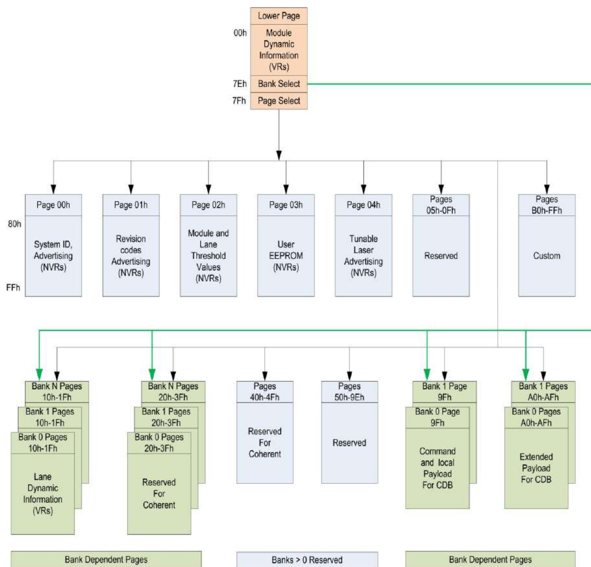
Figure5: Memory map
