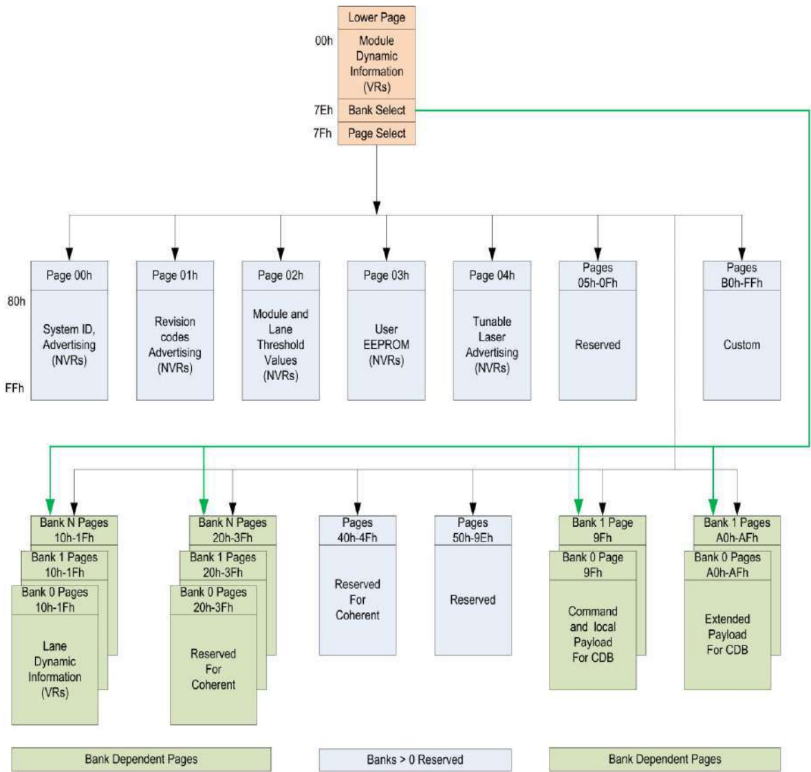
Figure5:Memory map
