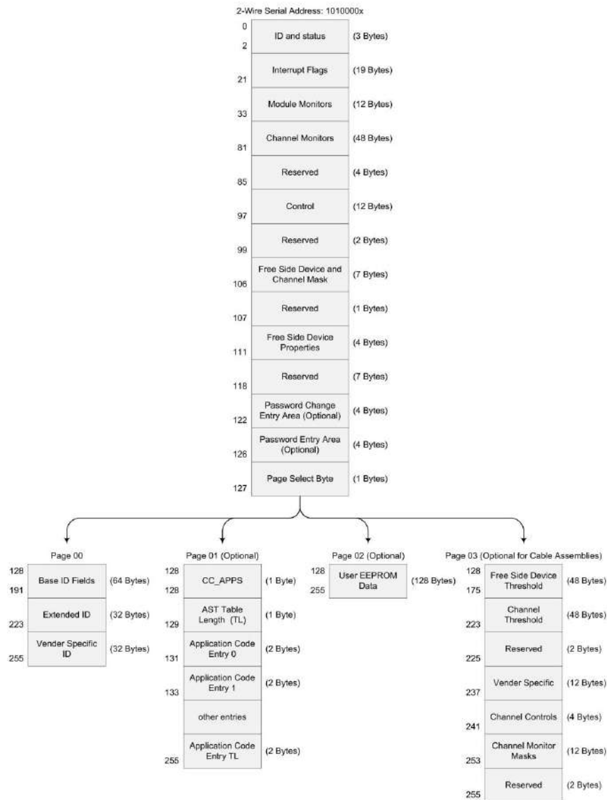
Figure4:Memory map
