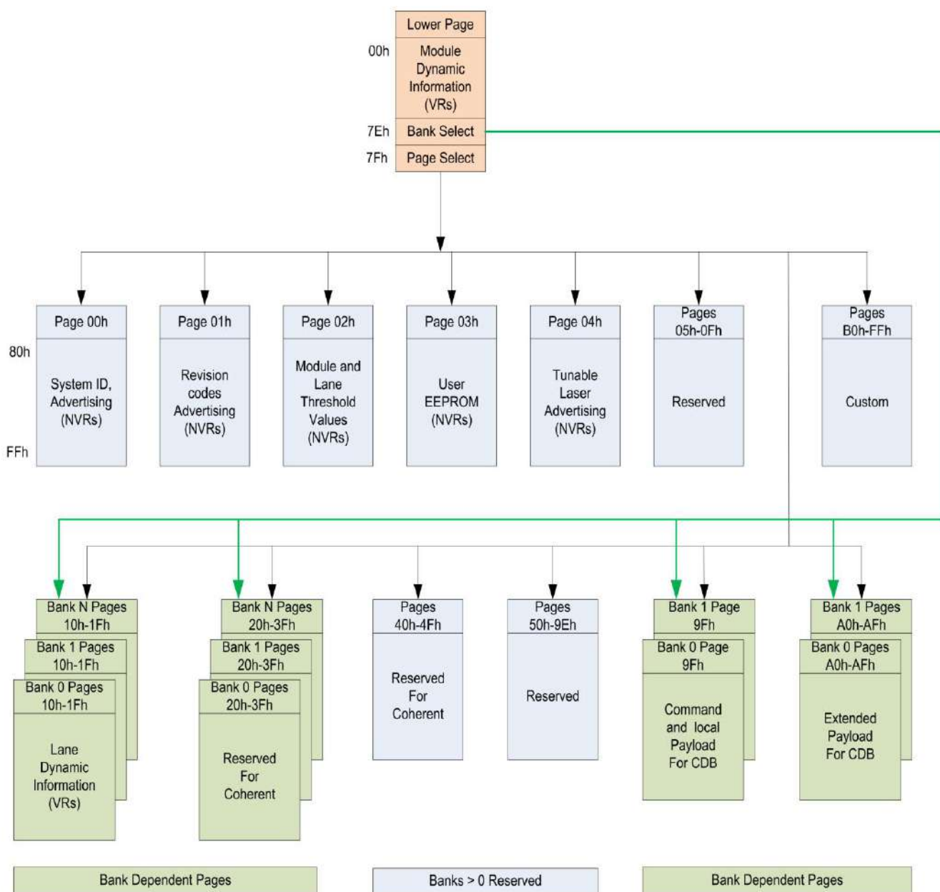
Figure5:Memory map
