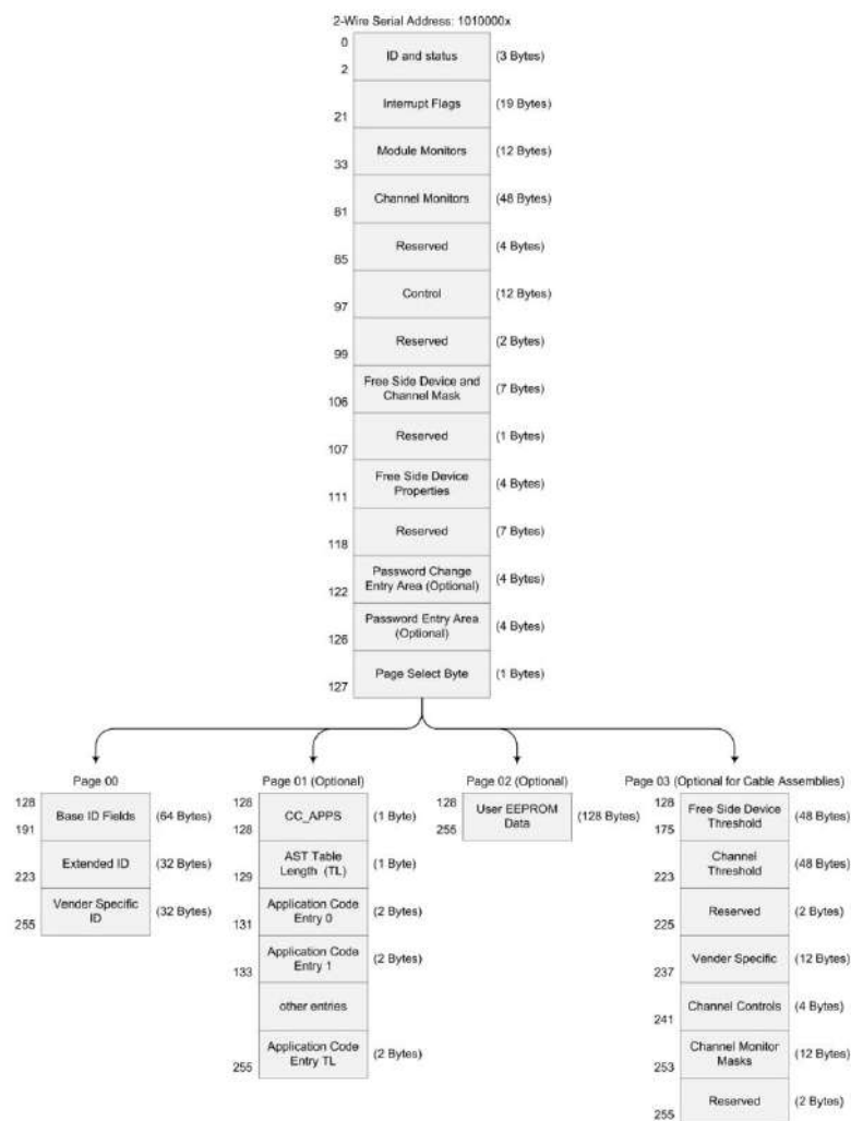
Figure4:Memory map
