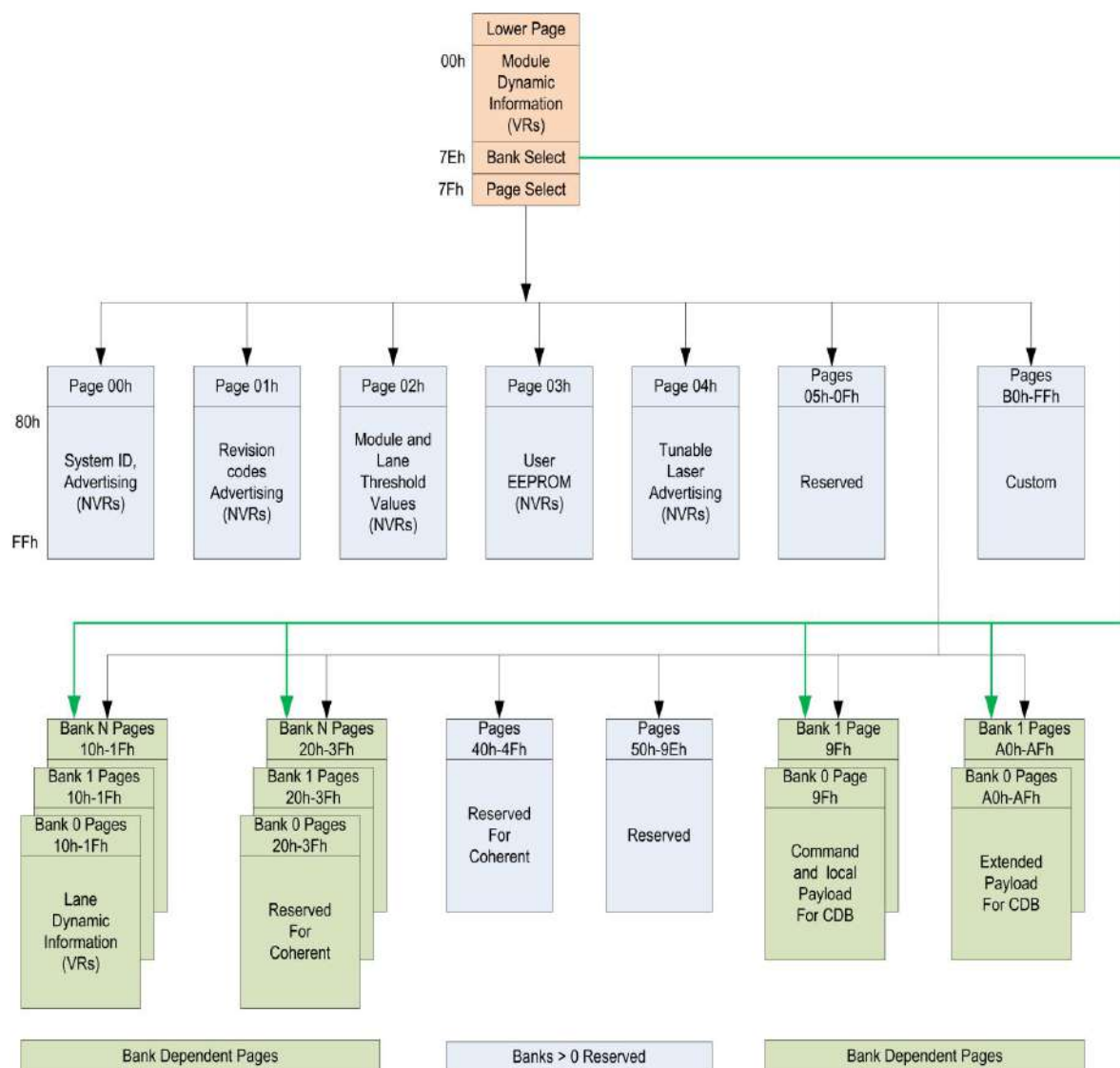
Figure5:Memory map
