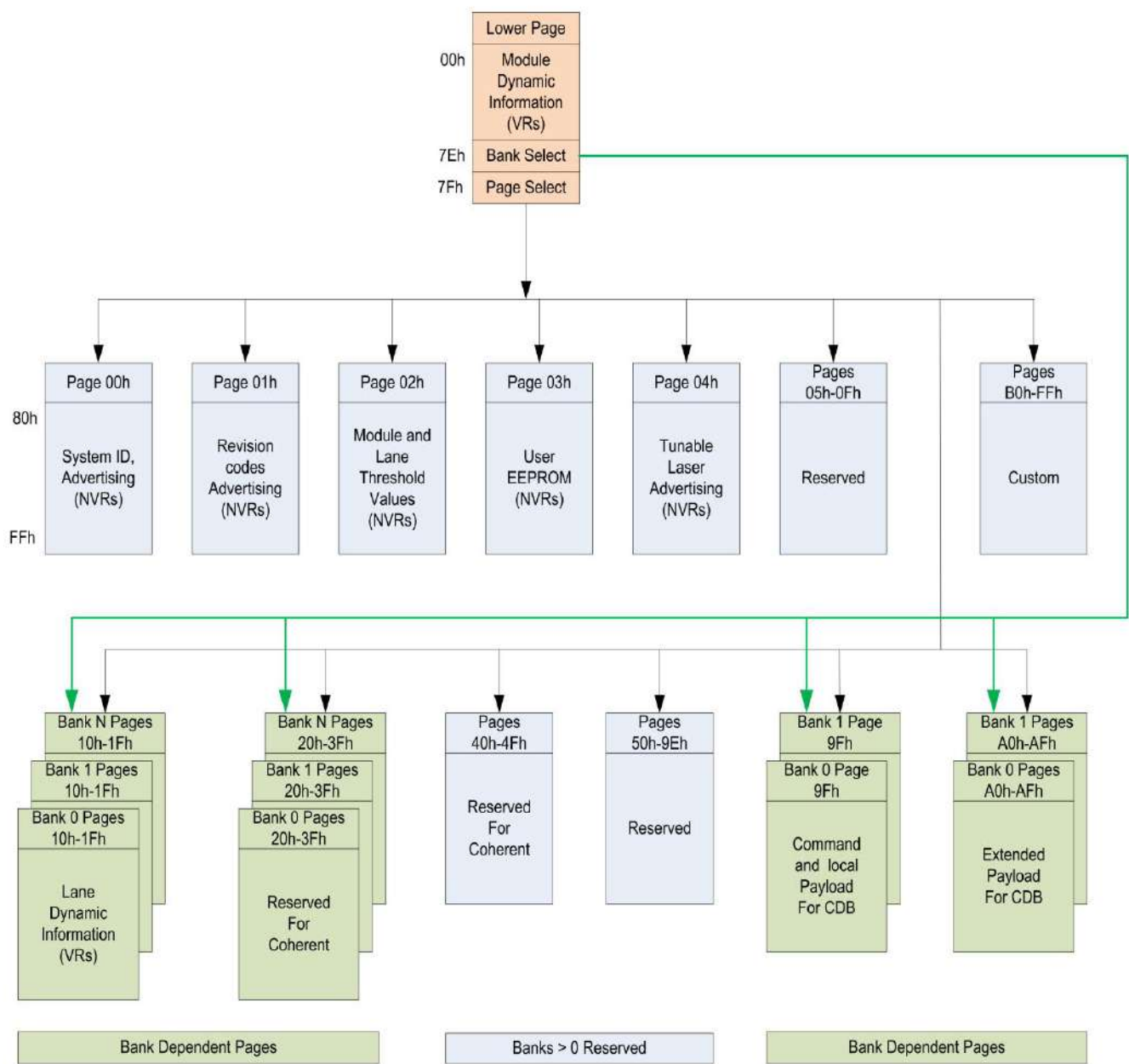
Figure4:Memory map
