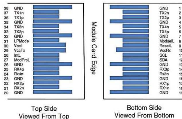
Figure3:Pin view
