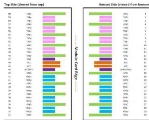
Figure3:Pin view
