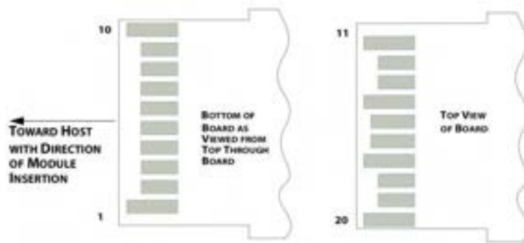
Figure3:Pin view
